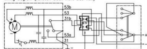
Wiring diagram (Junction block front side view)
